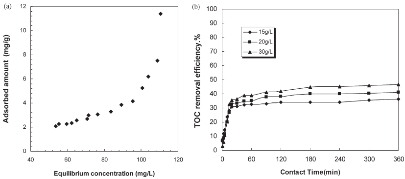
Figure 4. (a) Equilibrium adsorption of coal based PAC (Average initial TOC = 110 mg/L, mixing rate = 130 rpm, contact time = 72 hrs); (b) Kinetics adsorption of coal based PAC (Average initial TOC = 110 mg/L, mixing rate = 110 rpm, contact time = 6 hrs).
