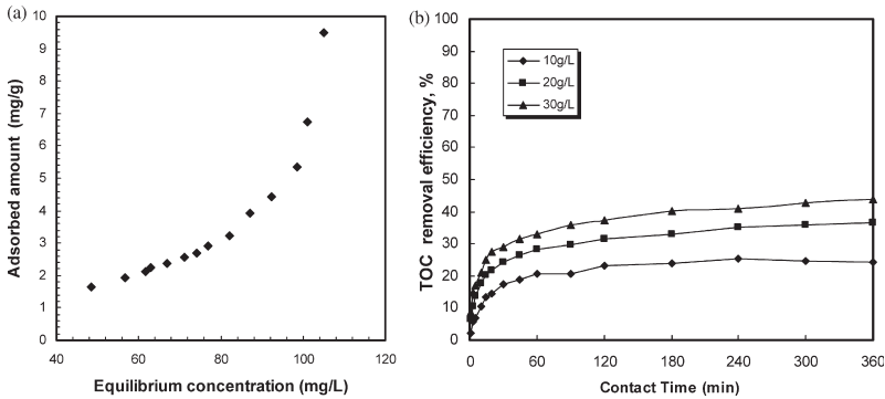
Figure 2. (a) Equilibrium adsorption of coal based GAC (Average initial TOC = 110 mg/L, mixing rate = 130 rpm, contact time = 72 hrs); (b) Kinetics adsorption of coal based GAC (Average initial TOC = 110 mg/L, mixing rate = 110 rpm, contact time = 6 hrs).
