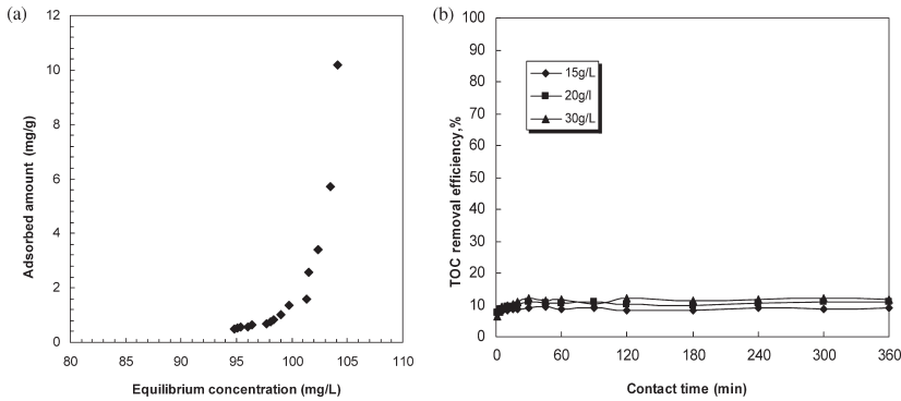
Figure 3. (a) Equilibrium adsorption of wood based PAC (Average initial TOC = 110 mg/L, mixing rate = 130 rpm, contact time = 72 hrs); (b) Kinetics adsorption of wood based PAC (Average initial TOC = 110 mg/L, mixing rate = 110 rpm, contact time = 6 hrs).
