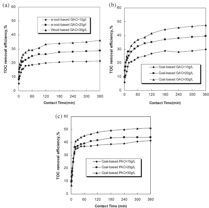
Figure 6. (a) Flocculation as pretreatment to wood based GAC for TOC removal from landfill leachate (Average initial TOC = 110 mg/L, mixing rate = 110 rpm, contact time = 6 hrs) (b) Flocculation as pretreatment to coal based GAC for TOC removal from landfill leachate (Average initial TOC = 110 mg/L, mixing rate = 110 rpm, contact time = 6 hrs); (c) Flocculation as pretreatment to coal based PAC for TOC removal from landfill leachate (Average initial TOC = 110 mg/L, mixing rate = 110 rpm, contact time = 6 hrs).
