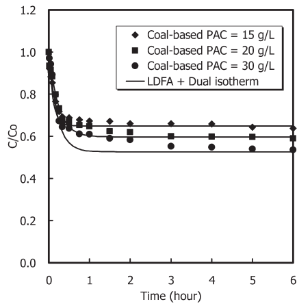
Figure 11. LDFA + Dual isotherm kinetics for TOC adsorption on coal-based PAC.
