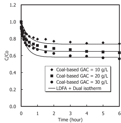
Figure 9. LDFA + Dual isotherm kinetics for TOC adsorption on coal-based GAC.
