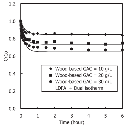
Figure 10. LDFA + Dual isotherm kinetics for TOC adsorption on wood-based GAC.
