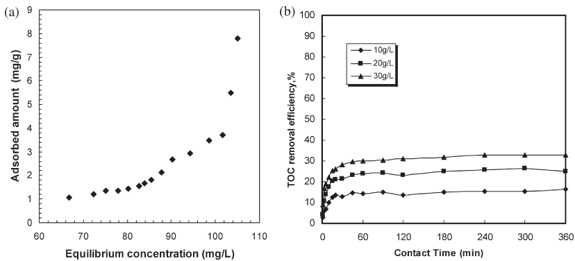
Figure 1. (a) Equilibrium adsorption of wood based GAC (Average initial TOC = 110 mg/L, mixing rate = 130 rpm, contact time = 72 hrs); (b) Kinetics adsorption of wood based GAC (Average initial TOC = 110 mg/L, mixing rate = 110 rpm, contact time = 6 hrs).
