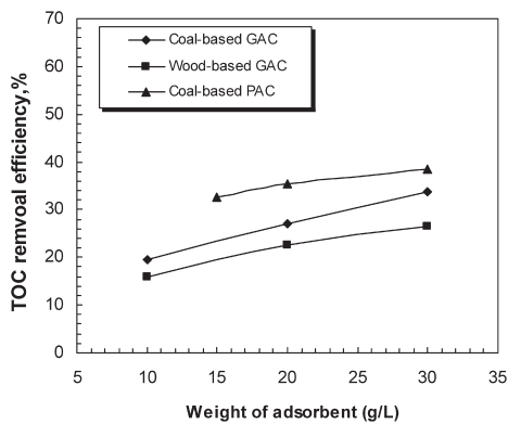
Figure 7. Combination of flocculation–adsorption for TOC removal from landfill leachate (rapid mixing gradient rate = 100 rpm, slow mixing gradient rate = 30 rpm, average initial TOC = 110 mg/L).
